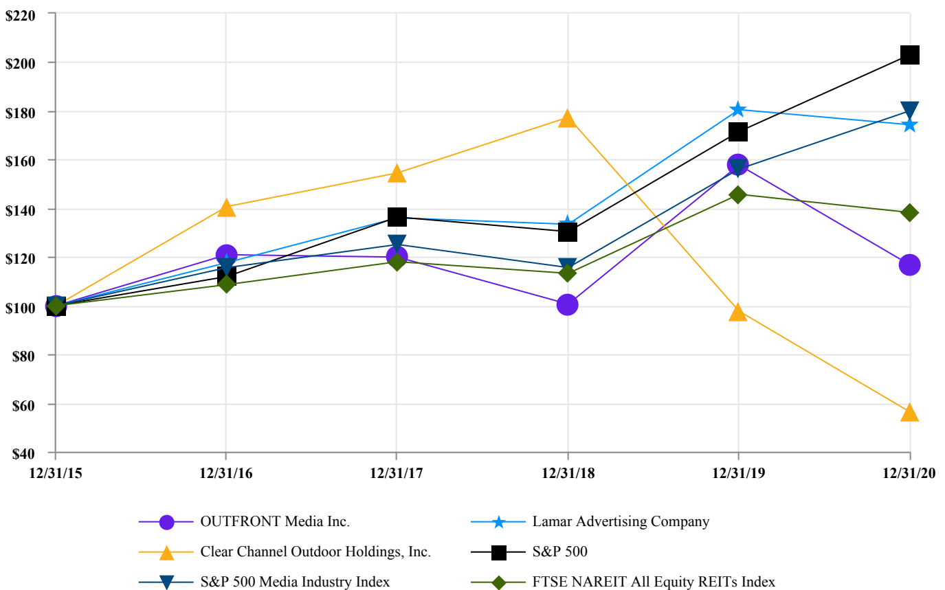
Performance Graph
