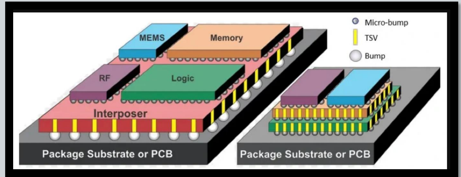
2.5D Architecture
