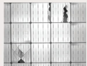
Crystalline Silicon Panel After Dynamic Load Test
