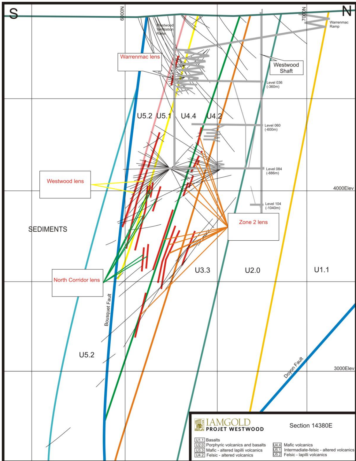
Figure 7.4: South-North cross-sectional interpretation of the Westwood deposit
