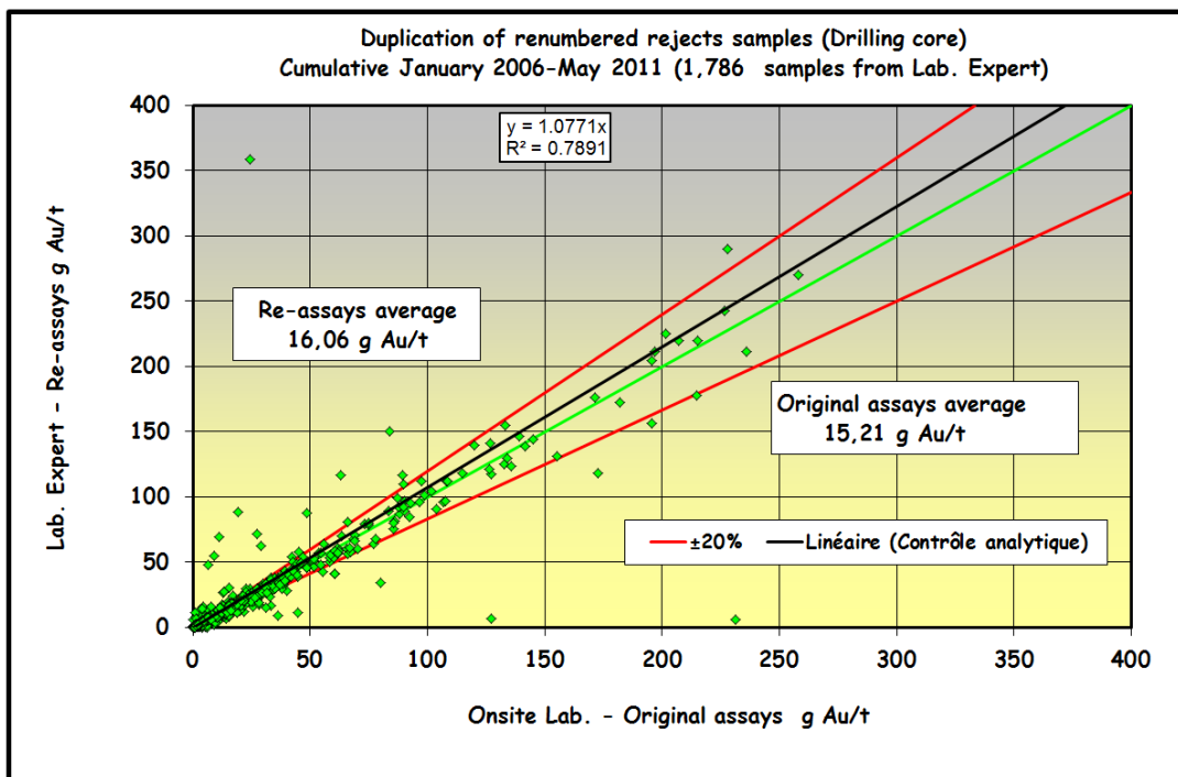
Figure 11.7 : Scatter Plot for two laboratories
