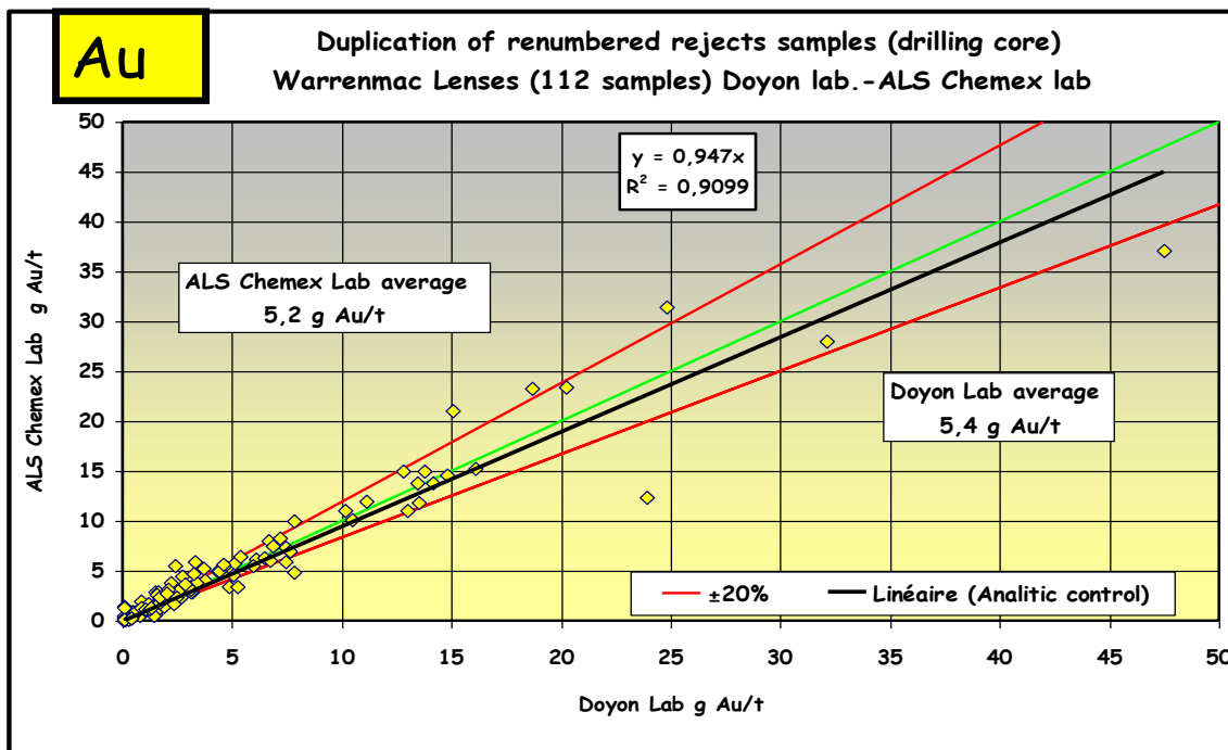
Figure 11.12 : Au Scatter Plot Results of both laboratories
