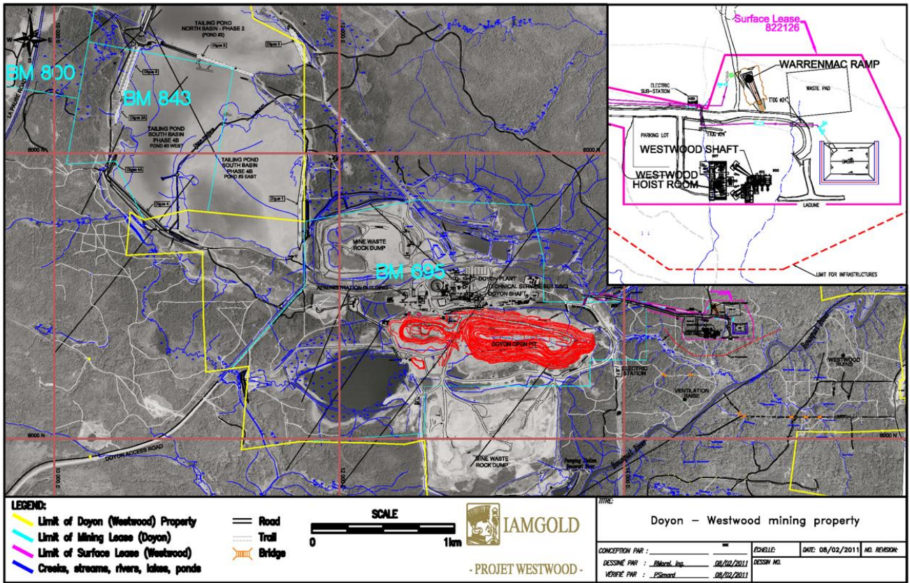
Figure 5.1: Doyon (Westwood) mining property
