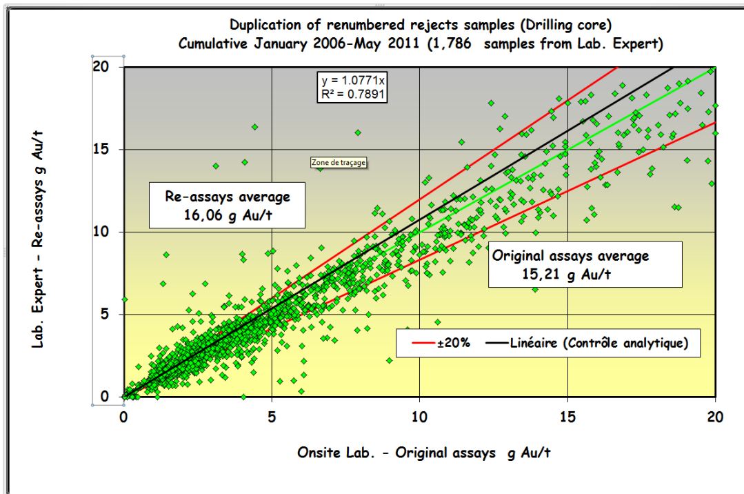
Figure 11.8 : Detailed Scatter Plot for two laboratories (0-20 g Au/t)
