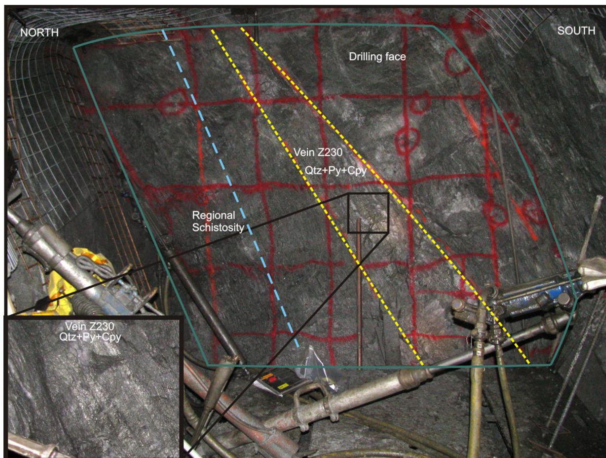
Figure 7.5: Zone 2 block-test mining on the Z230 Vein
