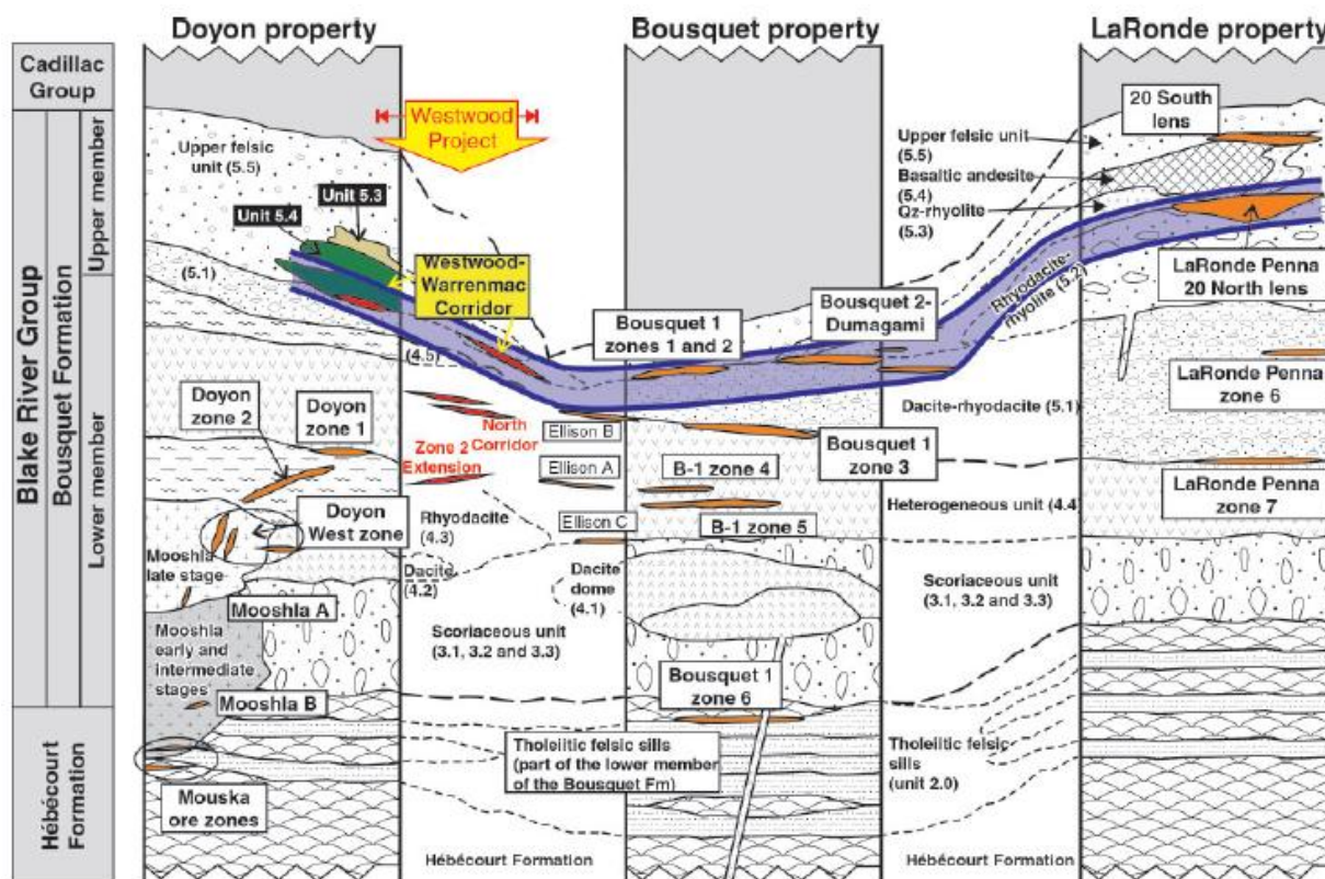
Figure 7.2: Doyon-Bousquet-La Ronde regional stratigraphy (from Mercier-Langevin et al. 2009)
