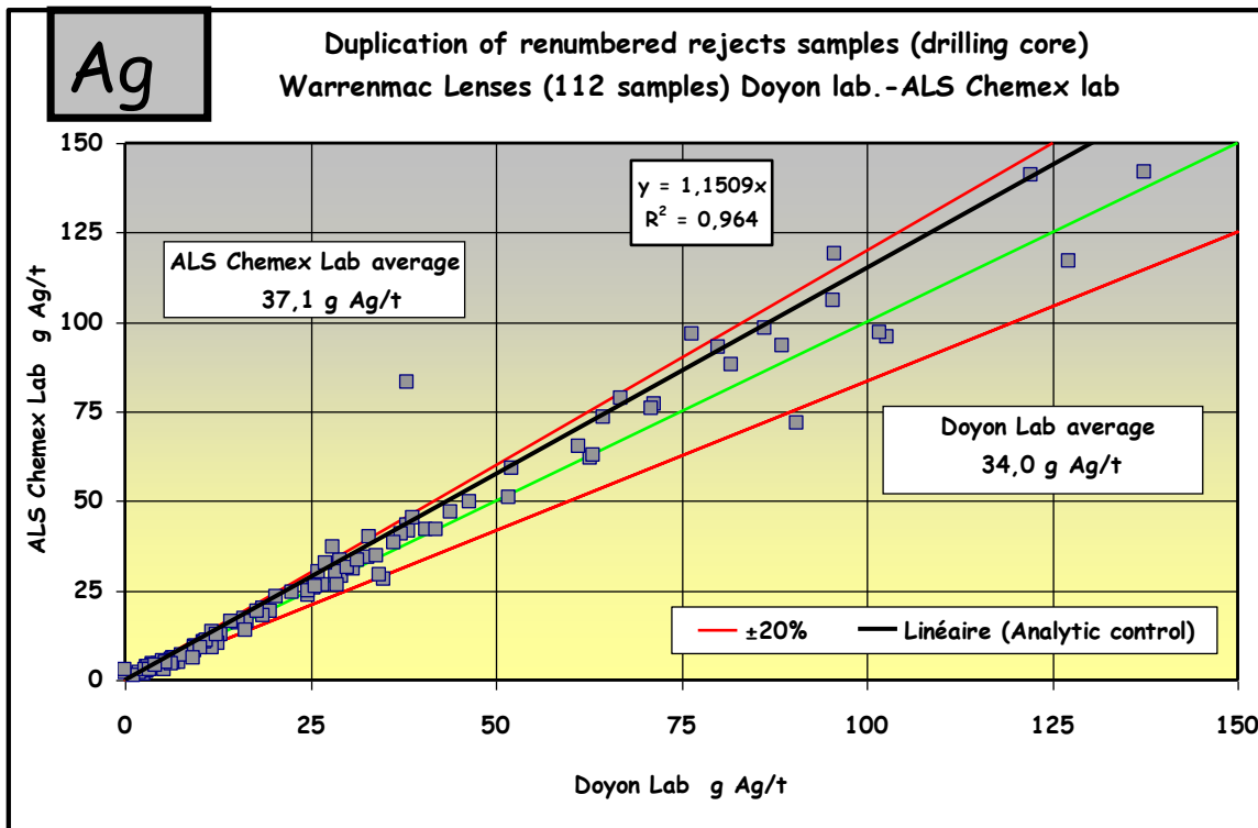
Figure 11.13 : Ag Scatter Plot Results of both laboratories
