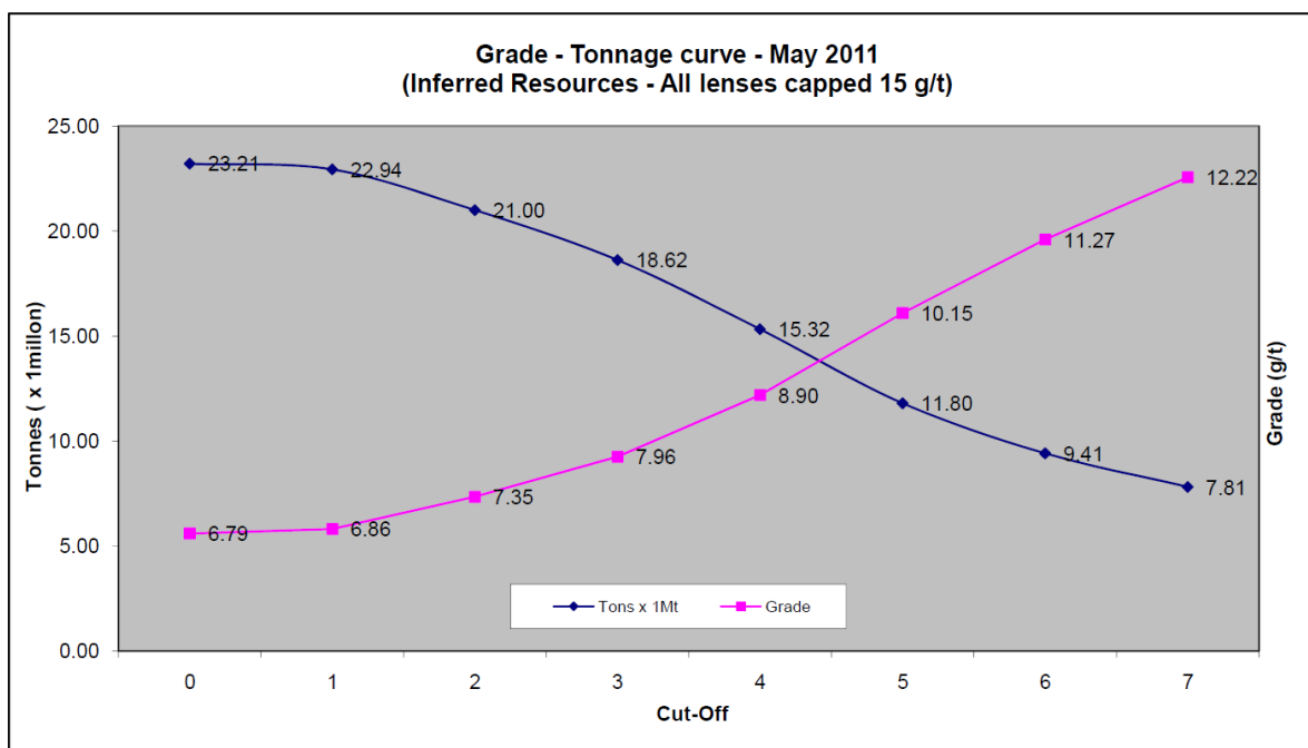
Figure 13.8: Grade Tonnage Curve - Inferred Resources – May 31 st 2011
