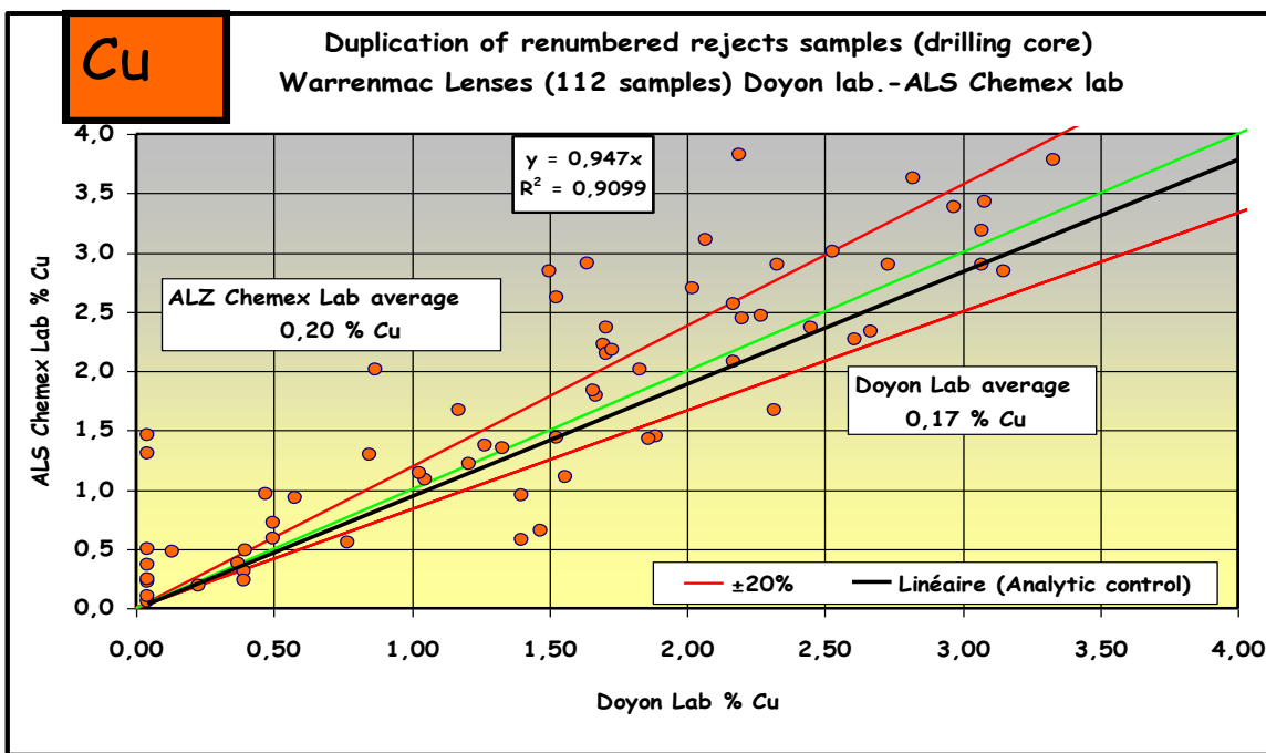
Figure 11.14 : Cu Scatter Plot Results of both laboratories
