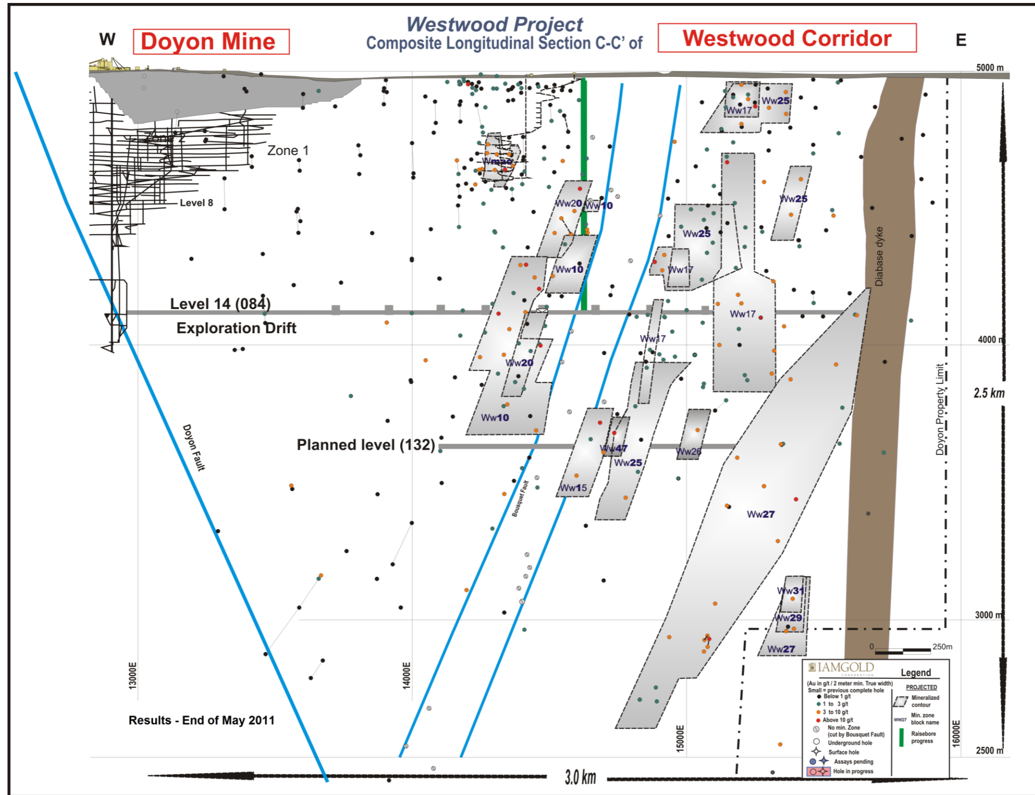
Figure 10.6: Composite longitudinal section C-C' of Westwood Corridor
