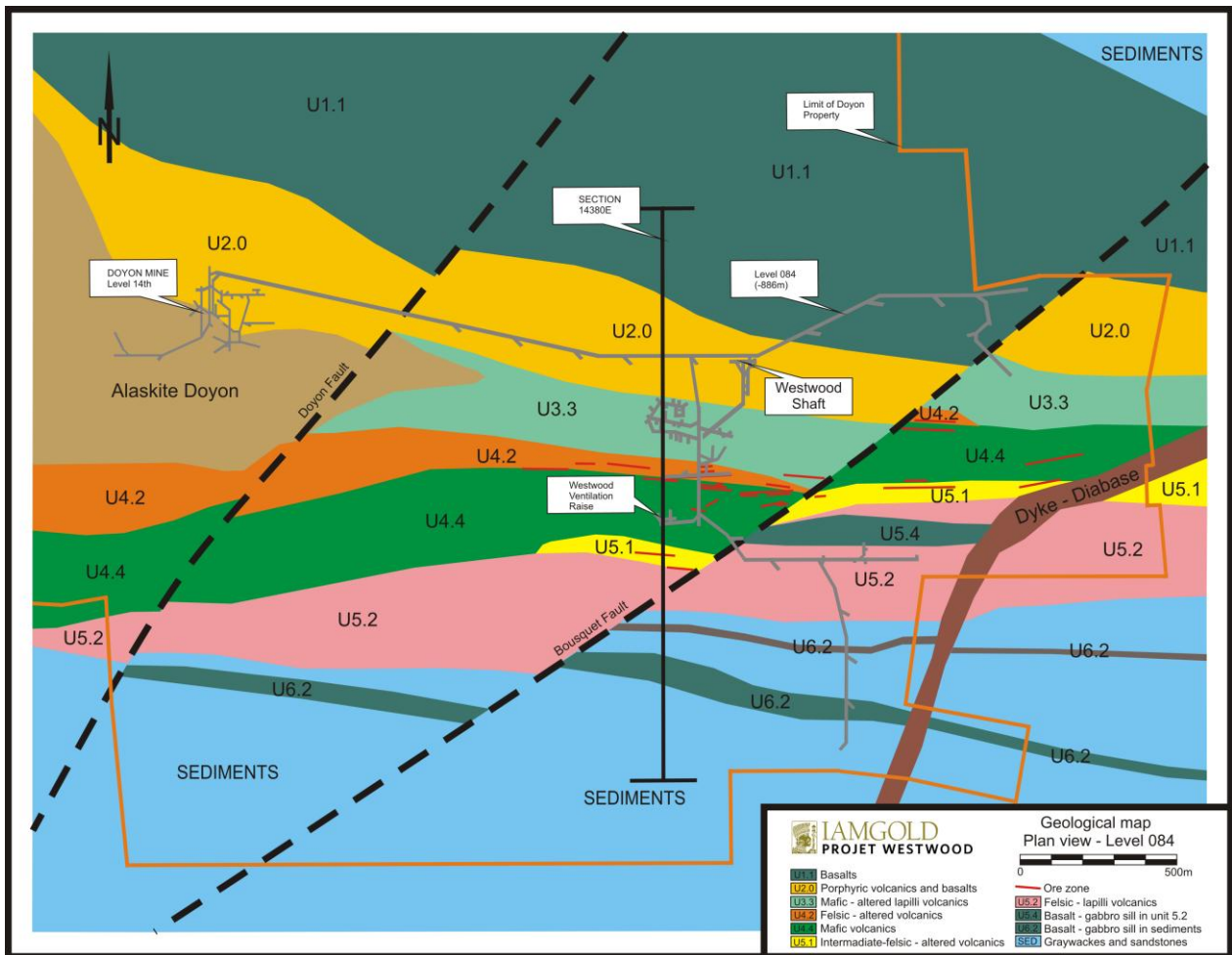
Figure 7.3: Geological Map – Plan view of Level 084
