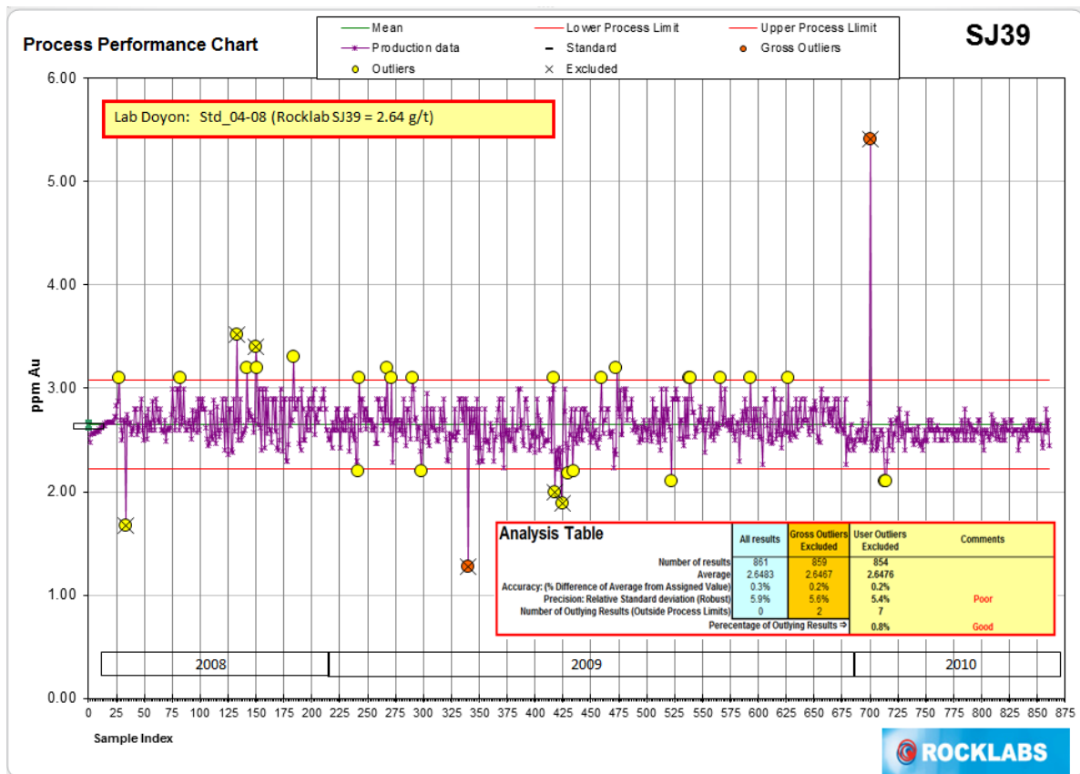
Figure 11.3 : STD4 Control Chart
