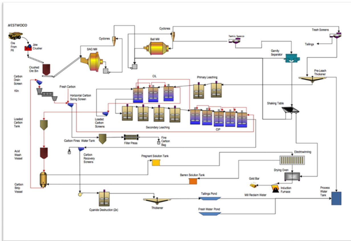
Figure 17-1: Grinding, Leaching, Adsorption and Stripping Circuit
