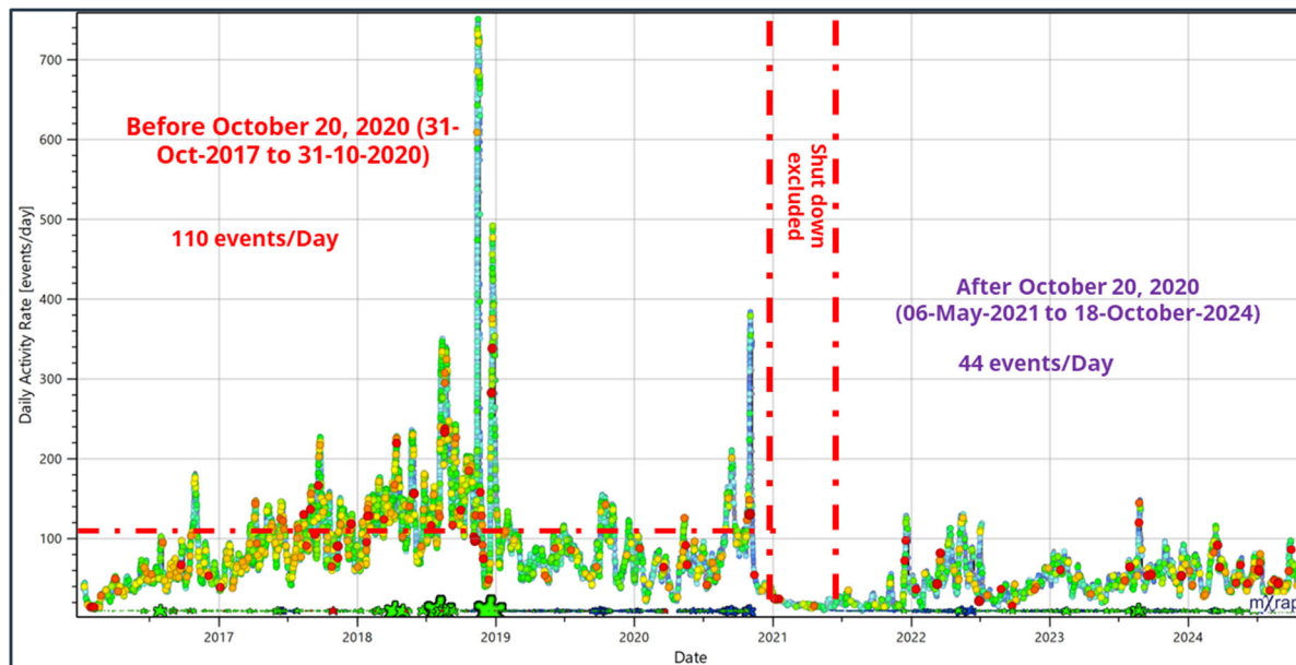
Figure 1-3: Westwood Seismic Events History
