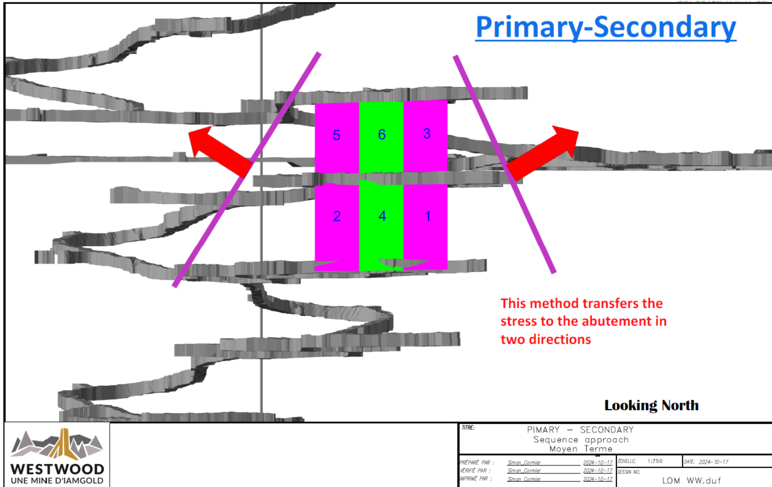
Figure 16-3: Former Mining Method, Westwood
